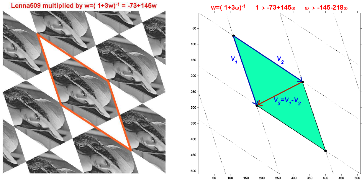
Fig. 4. The continuous model of the tiling produced by R_{1+3\omega} \in \mathbb{E}(509) .
