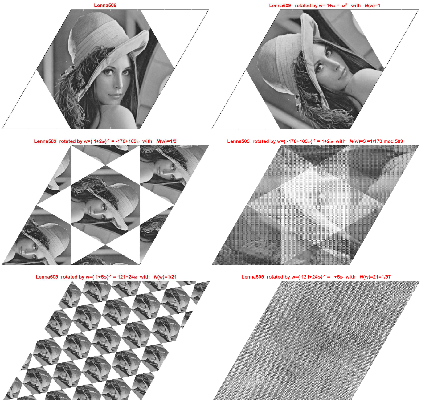
Fig. 3. Examples of Eisenstein rotations of a hexagonal image.
