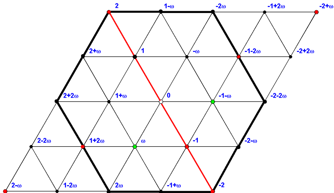
Fig. 2. The Eisenstein field \mathbb{E}(5) .
