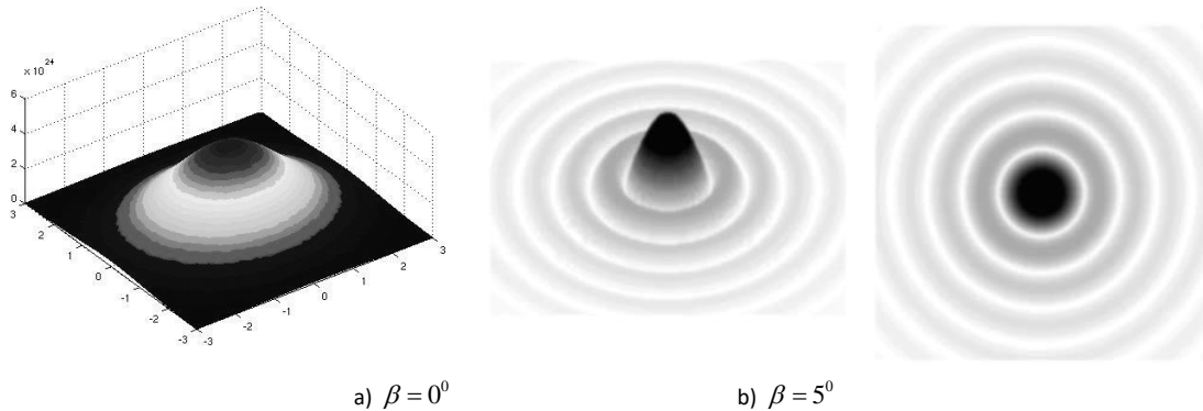
Fig. 5. The typical excitations a) in the form of 2-D Gaussian surface in the Fourier-Gaussian metamedium and b) in the form of a wave packet in the Schrödinger-Euclidean metamedium ( t_k = 128, \beta = 5^0 ).
