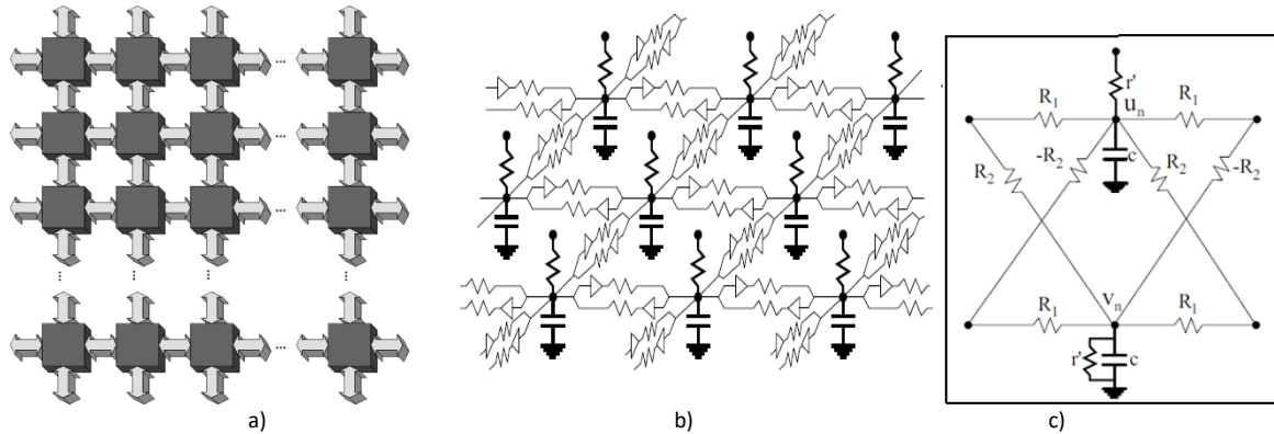
Fig. 3. a) The 2-D cellular automaton (the Schrödinger metamedium) and b) its equivalent electrical circuit in the form of spatially distributed RC-circuit that simulates a simple diffusion media, c) a single cell \text{Aut}(n, m) of the 2-D cellular automaton in form of a 2-channel (complex) filter.
