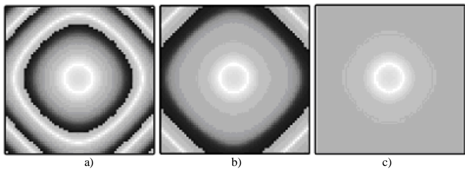
Fig. 10. The excitation of three Schrödinger-Yaglom metamaterials at the moment t_k = 128 for three values of the parameter k : a) k = -0,25 , b) k = -0,05 , c) |k| \rightarrow 0 for identical values \arg\{\mathbf{D}\} = 40.5^\circ and |\mathbf{D}| = 0.07 .
