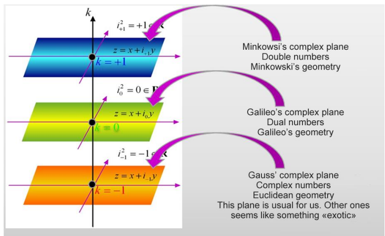
Fig. 9. In every plane, that crosses the vertical of the k -parameter axis, there is an algebra A_2(\mathbf{R} | i_k) := \{z = a + i_k b | a, b \in \mathbf{R}\} . Three planes that cross this axis at three points k = \mp 1, 0 represent three algebras of complex numbers that were considered before.
